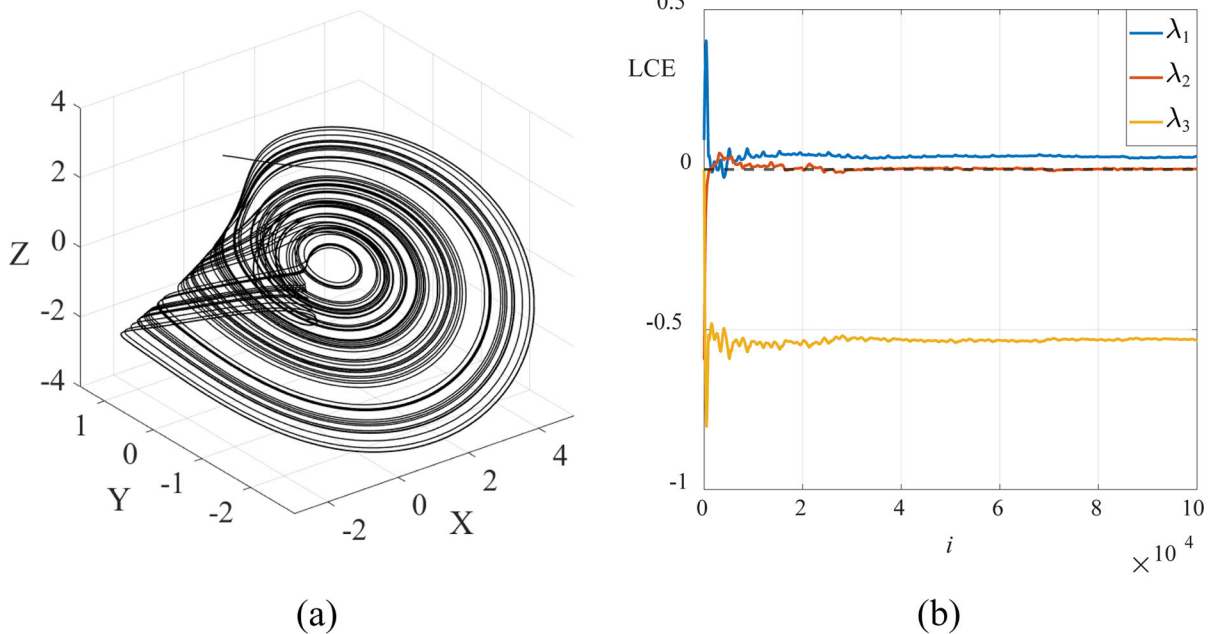
Fig. 3 a Phase portrait and b LCE of chaotic attractor #1
