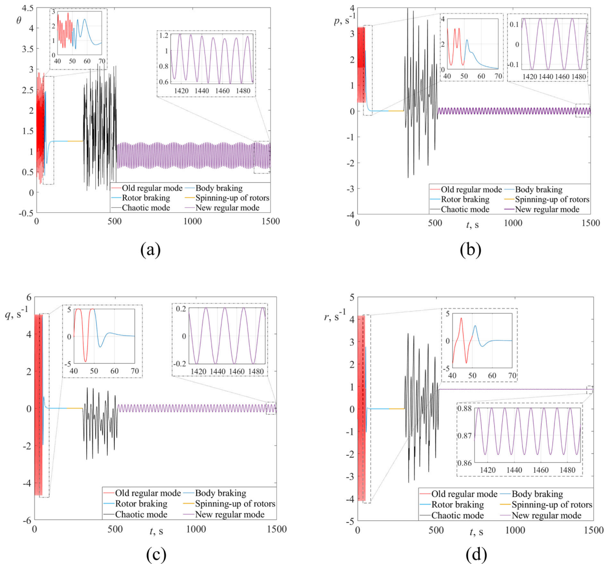
Fig. 5 Dependence of (a) nutation, (b) p velocity component, (c) q velocity component, and (d) r velocity component on time
